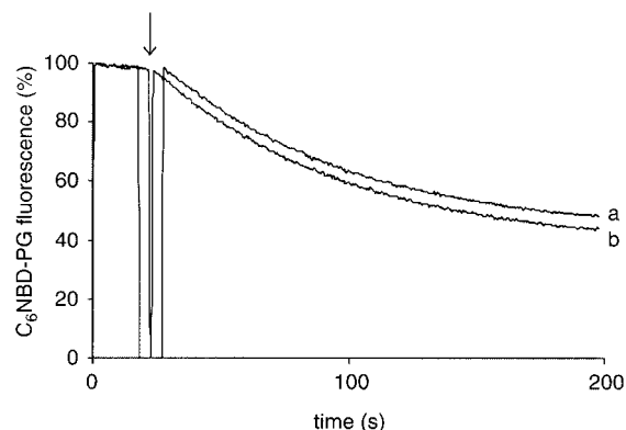
FIGURE 1: On-line fluorescence measurements of the dithionite reduction of C 6 NBD-PG (0.2% of total PL) present in both leaflets of vesicles, composed of E. coli phospholipids, without (a) and with (b) the model peptide KALP31 incorporated at a 1:2000 peptide:PL molar ratio. At the time point indicated by the arrow, sodium dithionite was added to a final concentration of 8 mM to the vesicles which were present at a concentration of \sim 150 \mu\text{M} (PL). The fluorescence is presented as the percentage of the initial fluorescence.
